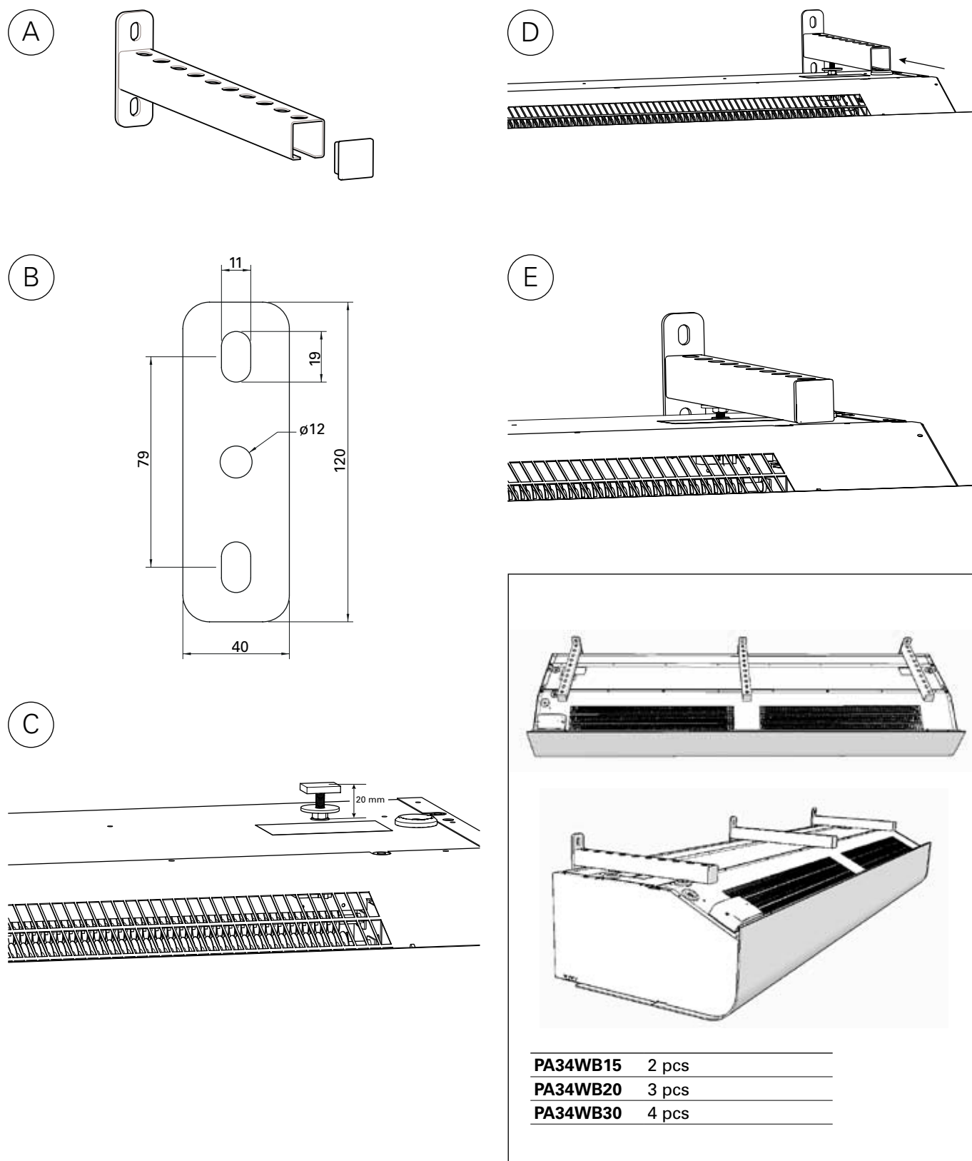
Fig. 5: Mounting with wall brackets (PA34WB).
